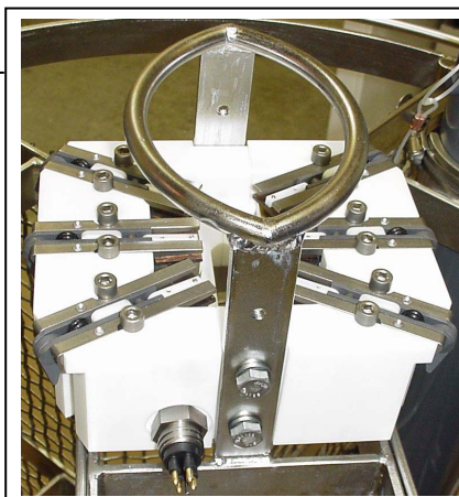
SBE 55 ECO Water Sampler with two 3-position lanyard release modules
