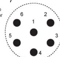
Optional Wet-Pluggable Connector MCBH-6MP (WB), TI (3/8" length base, 1/2-20 thread)
