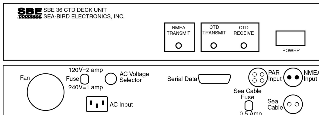
SBE 36 Front Panel
