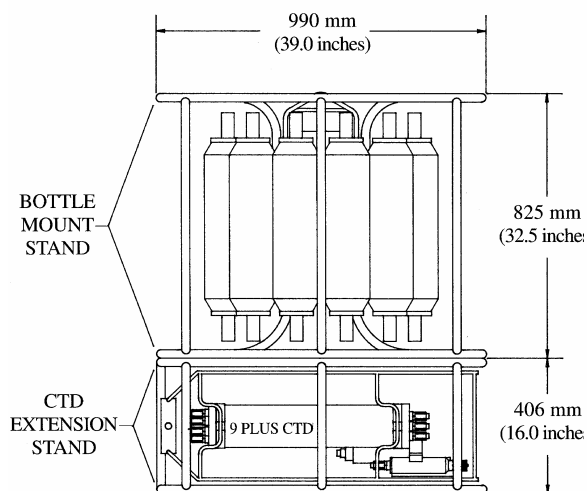
Full Size Carousel (12-bottle, 5-liter shown)
