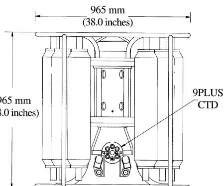
Compact Carousel with 9plus
